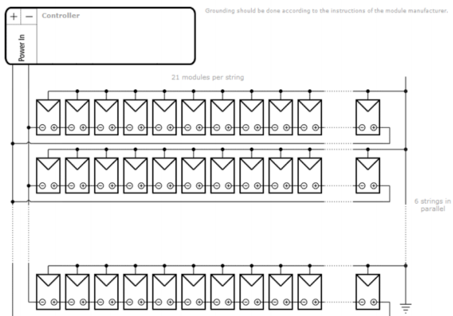
Wiring diagram
