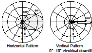
1920 – 2180 MHz: +45°/-45° Polarization
