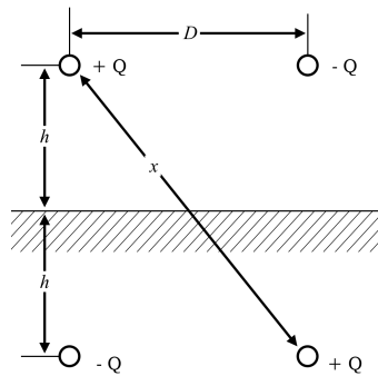
Slika 3.5.2: SGU model [13]
