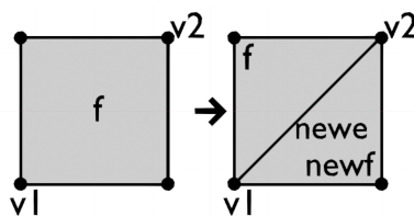
Sl. 4.9: ManifoldMakeEdge
