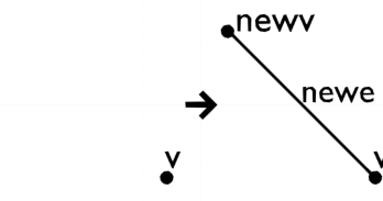
Sl. 4.8: MakeEdgeVert
