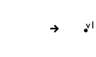
Sl. 4.6: MakeVert
