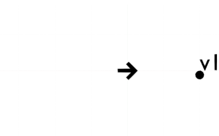
Sl. 4.6: MakeVert
