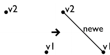
Sl. 4.7: MakeEdge
