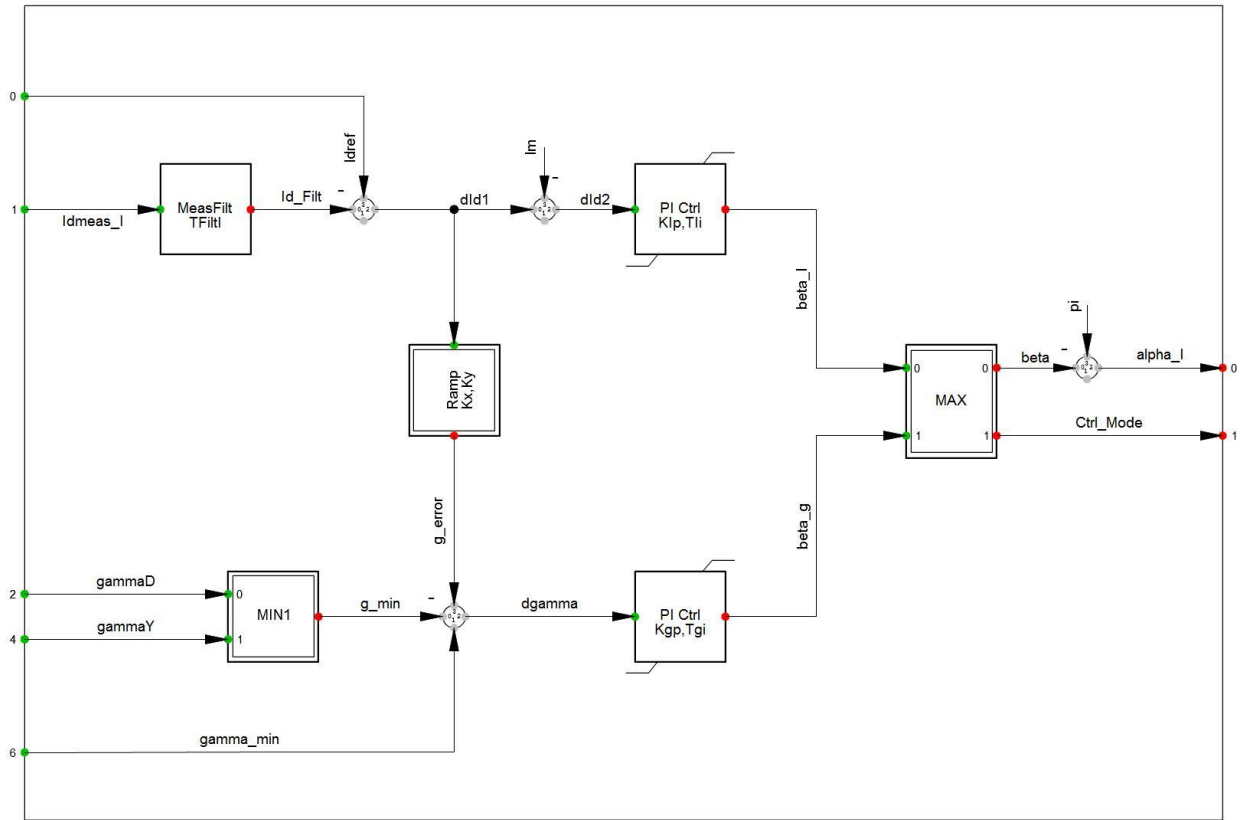
Inverter Controller: Inverter Controller
