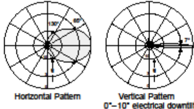
1850 – 1990 MHz: +45°/–45° Polarization
