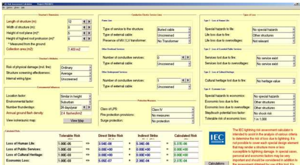
Slika 4.9. Proračun rizika udara munje prema Software-u IEC Risk Assessment Calculator [17]
