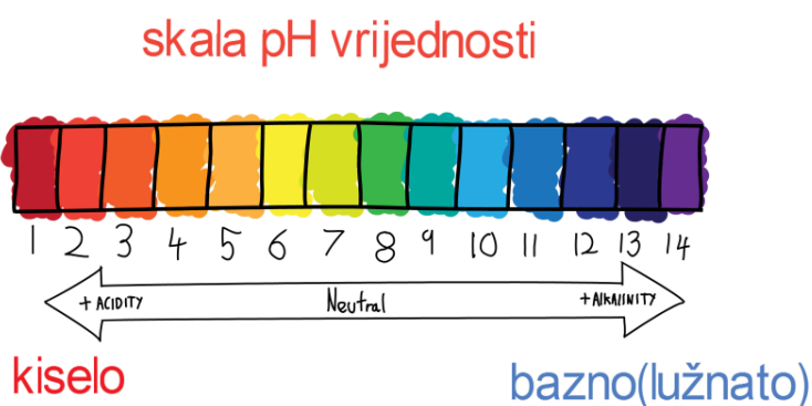
Sl. 3.4 pH skala [12]
